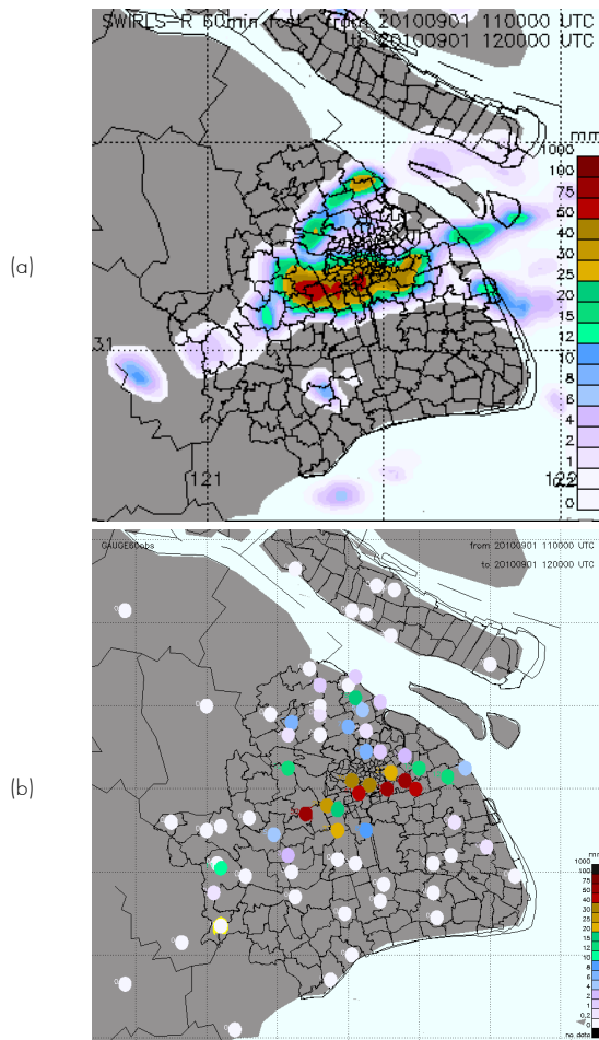
Fig. 5 Real-time example of localized heavy rain forecast for Shanghai on 1 September 2010: (a) 1-hour nowcast by SWIRLS issued at 19:00 local time; (b) actual 1-hour accumulated rainfall ending at 20:00 local time reported by raingauges.
