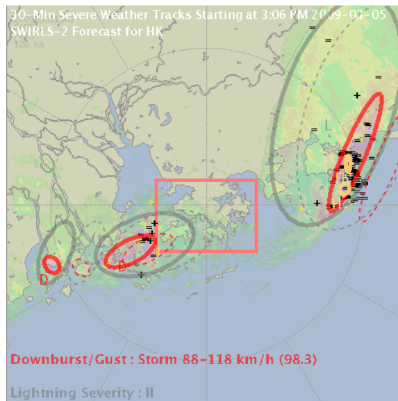
Fig. 3 Severe Weather Map of SWIRLS issued at 3:06 pm on 5 March 2009. Red and grey ellipses indicate the analyzed threat areas of severe wind gust and CG lightning respectively. Dashed ellipses indicate the forecast positions of the threat areas in 30 minutes. Small yellow "o", black "=" and black "+" symbols mark the locations of actual cloud-to-cloud, negative CG and positive CG lightning respectively.
