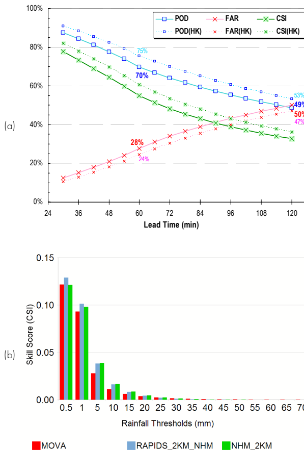
Fig. 6 Verification results of SWIRLS QPF for 2010-2011 over the “PRD” domain: (a) POD (blue), FAR (red) and CSI (green) in the first two hours of prediction at the 0.5-mm threshold (note: dashed curves refer to the smaller “HK” domain); (b) CSI at the lead time of 6 hours (red histograms labeled “MOVA”). Also shown in (b) are CSIs of the blended forecast from RAPIDS (blue) and the underlying 2-km NHM QPF (green).
