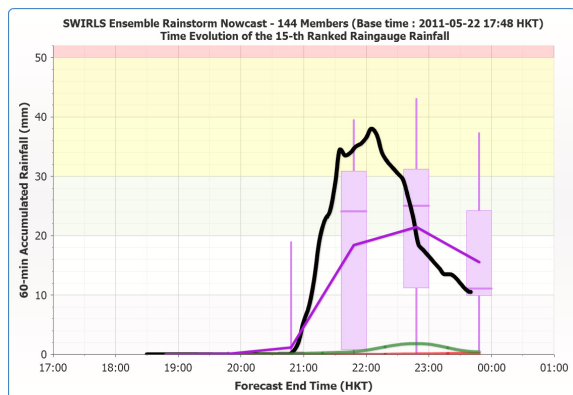
Fig. 7 Illustrative example of ensemble rainstorm nowcasting. The y-axis refers to the value of the key rainfall parameter (i.e. the “15-th ranked raingauge rainfall”) most critical to the Observatory’s rainstorm warning criteria. Different background colours indicate different warning thresholds. The black curve and the purple box-whisker diagrams represent respectively the actual and predicted values of the key rainfall parameter. Also shown are the existing extrapolation nowcasts based on TREC (green curve) and MOVA (red curve).
